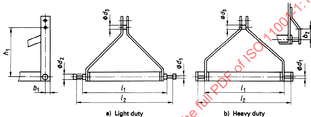
Figure 2 — Dimensions associated with implement
