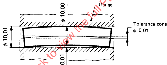
FIGURE 5 c) – Maximum material pin ( \phi 10) shown in gauge – Effective straightness tolerance \phi 0,01
