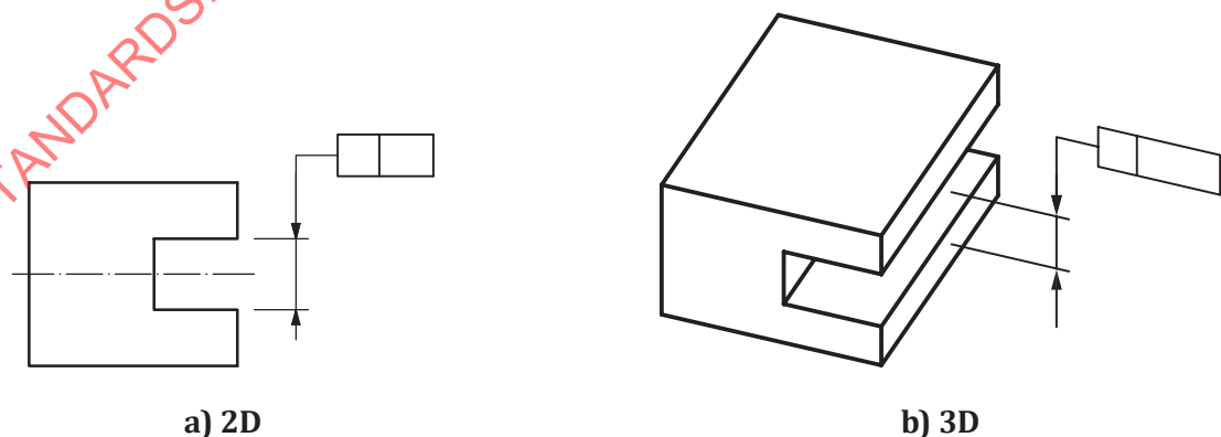
Figure 6 — Indication of derived feature specification
