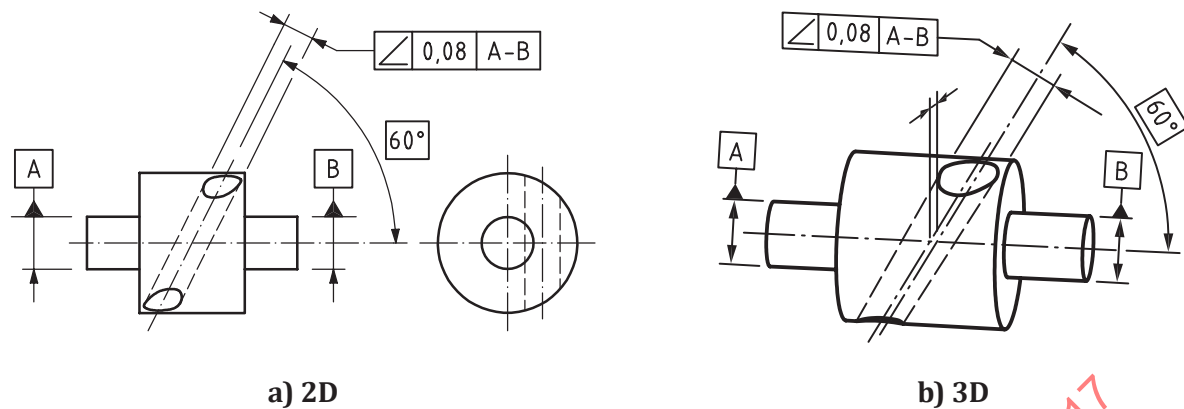
Figure 140 — Angularity indication
