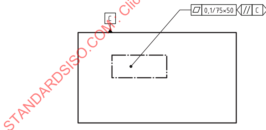
Figure 67 — Indication of an areal restricted specification
