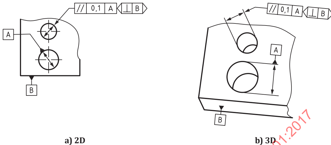
Figure 114 — Parallelism indication
