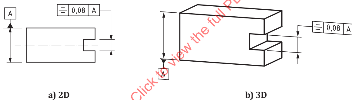
Figure 169 — Symmetry indication
