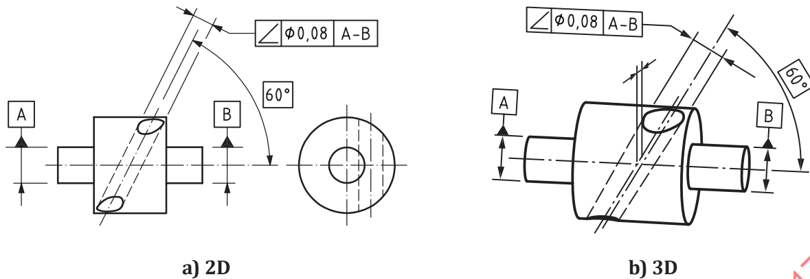
Figure 142 — Angularity
