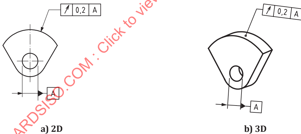
Figure 176 — Circular run-out indication
