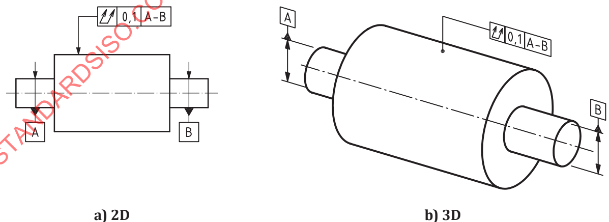
Figure 184 — Total run-out indication
