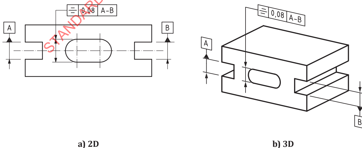
Figure 170 — Symmetry indication
