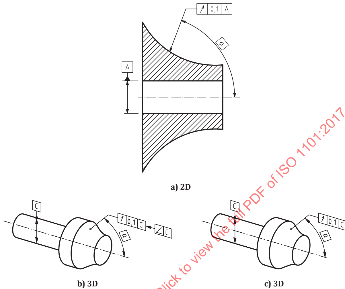
Figure 85 — Drawing indication
