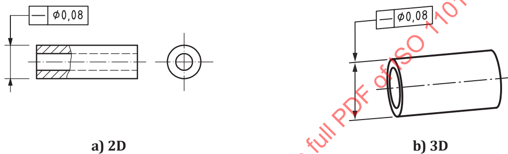
Figure 94 — Straightness indication
