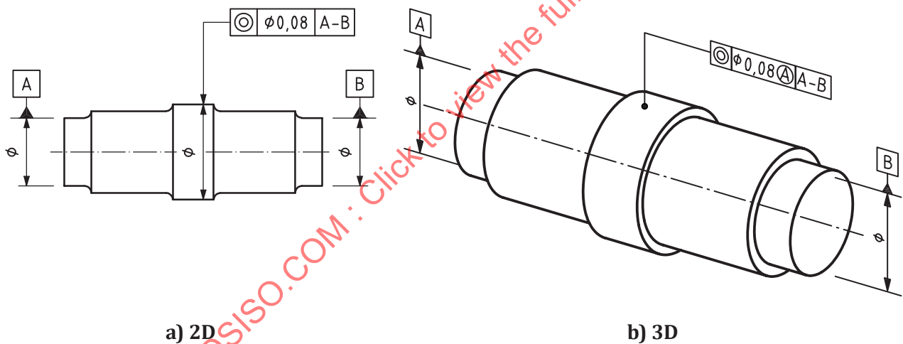
Figure 165 — Coaxiality indication
