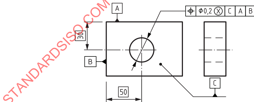
Figure 33 — Maximum inscribed associated toleranced feature — Drawing indication
