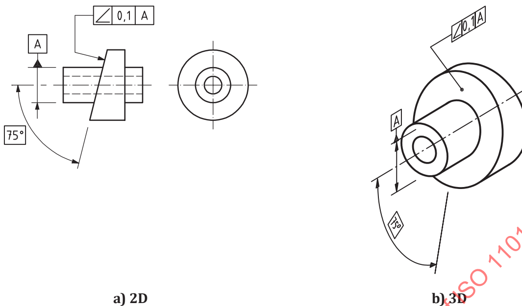
Figure 146 — Angularity indication
