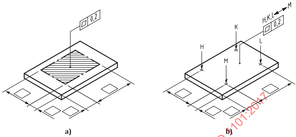
Figure 57 — Indication of restricted area
