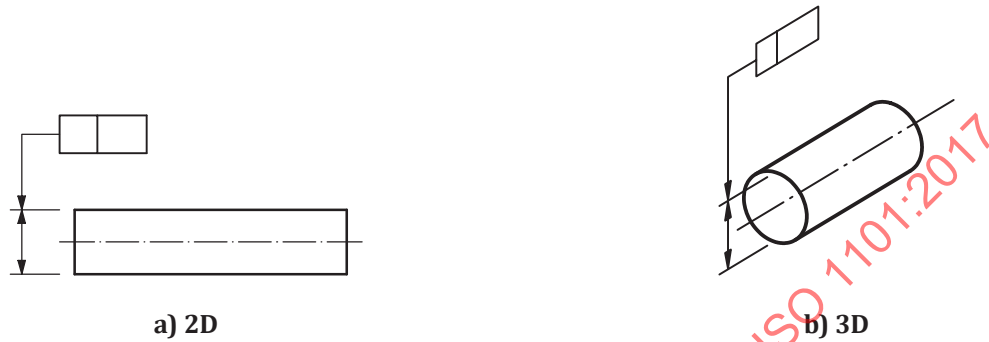
Figure 4 — Indication of derived feature specification
