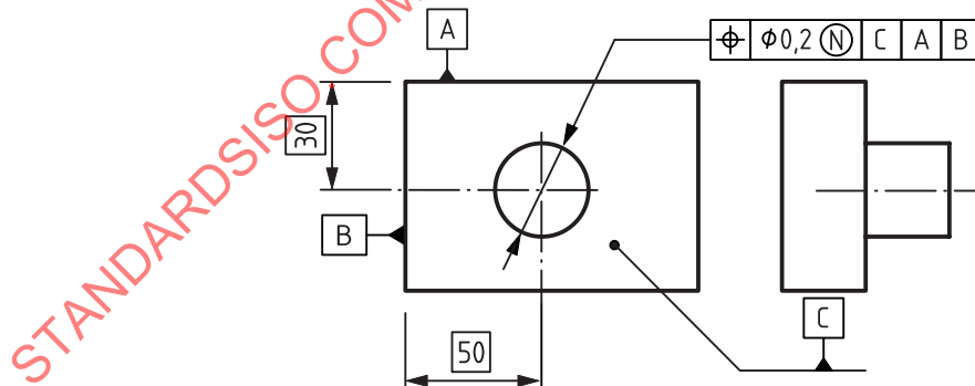
Figure 29 — Minimum circumscribed associated tolerated feature — Drawing indication
