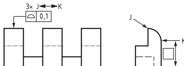
Figure 63 — Indication of several compound toleranced features
