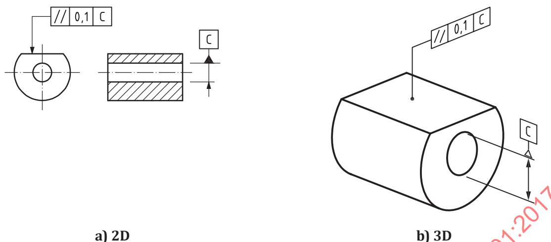
Figure 124 — Parallelism indication
