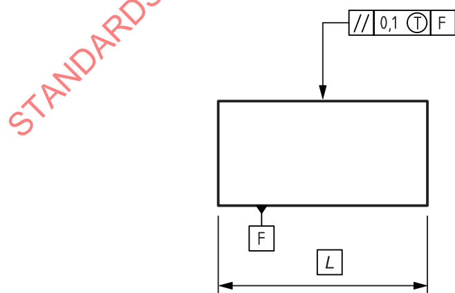
Figure 31 — Tangent associated tolerated feature — Drawing indication
