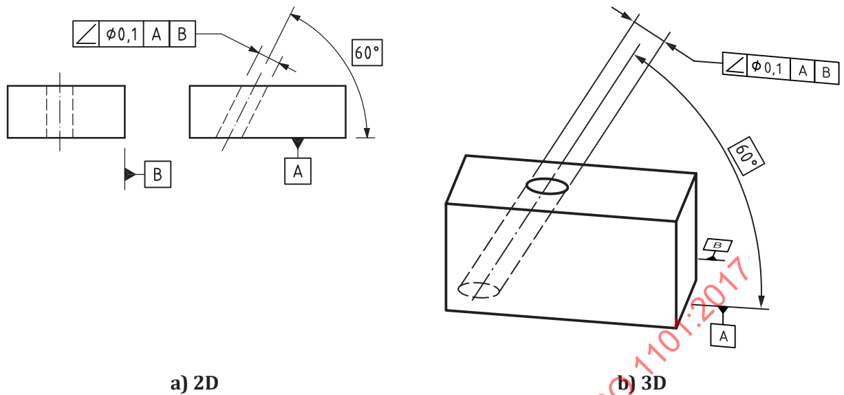
Figure 144 — Angularity indication
