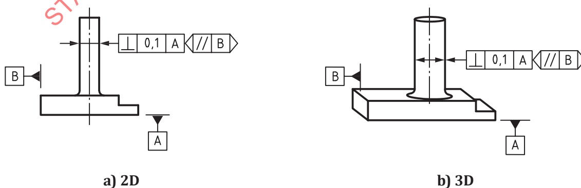
Figure 130 — Perpendicularity indication
