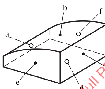
Figure 53 — All around drawing indication
