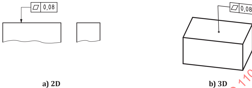
Figure 96 — Flatness indication
