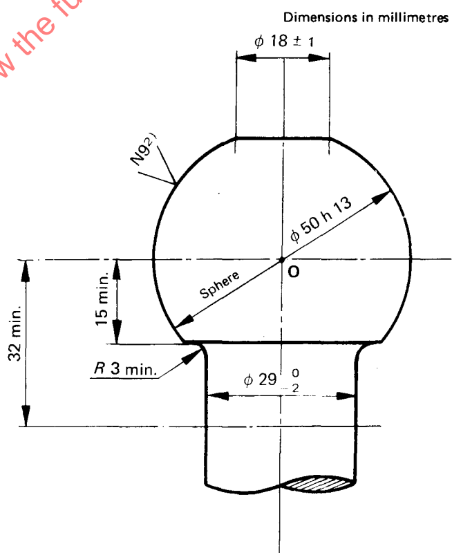
FIGURE 1 — Dimensions and tolerances of the coupling ball
