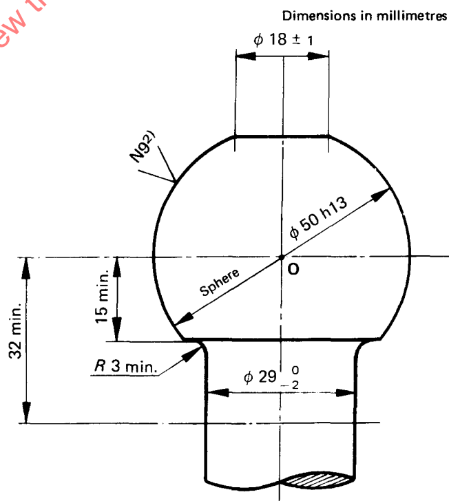
FIGURE 1 — Dimensions and tolerances of the coupling ball
