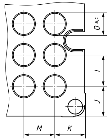
d) 40 cavity nest for compatible barrel sizes 20 ml
