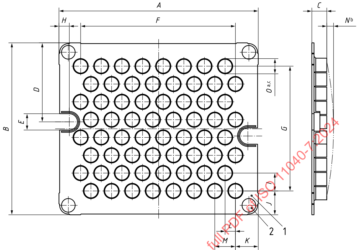
a) 64 cavity nest for compatible barrel sizes 5 ml
