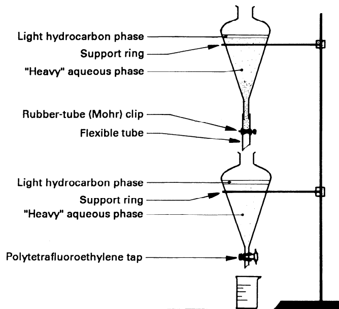
Figure 1 — Separation apparatus
