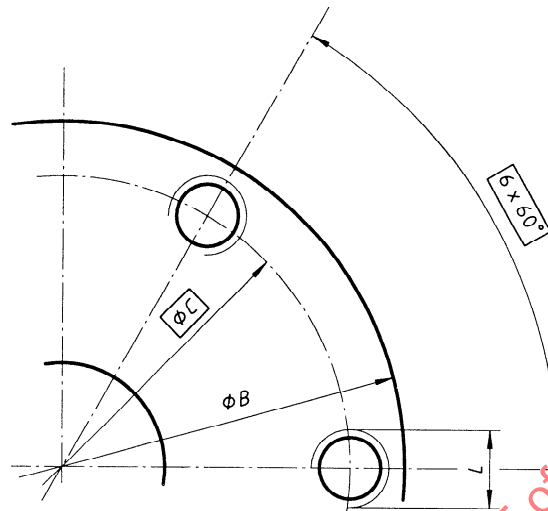
Figure 2 — 6 hole pattern
