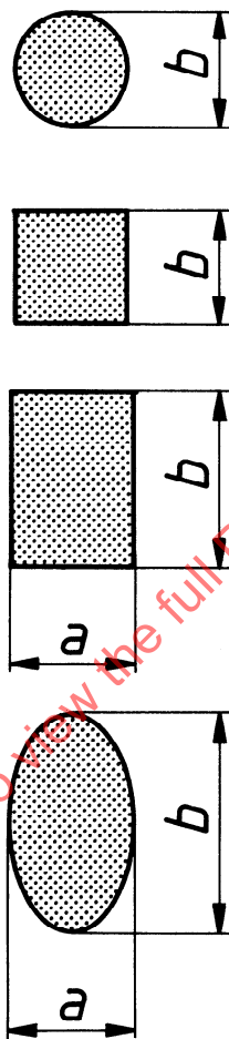
Figure 1 — Determination of effective focal spot size from projected focal spot images of various shapes [effective width of focal spot, f = (a + b)/2 ]
