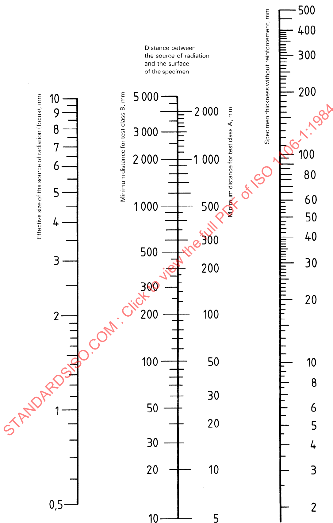
Figure 3 — Nomogram for the determination of the minimum distance between the source of radiation and the surface of the specimen in terms of the specimen thickness and the effective size of the source of radiation
