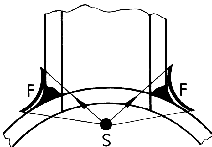
Figure 6 — Film outside, source of radiation inside (source central)
