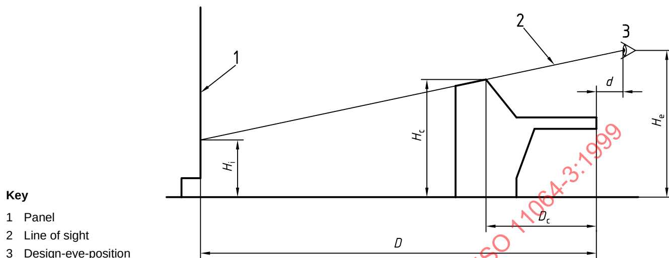
Figure 7 — Control workstation height and view over
