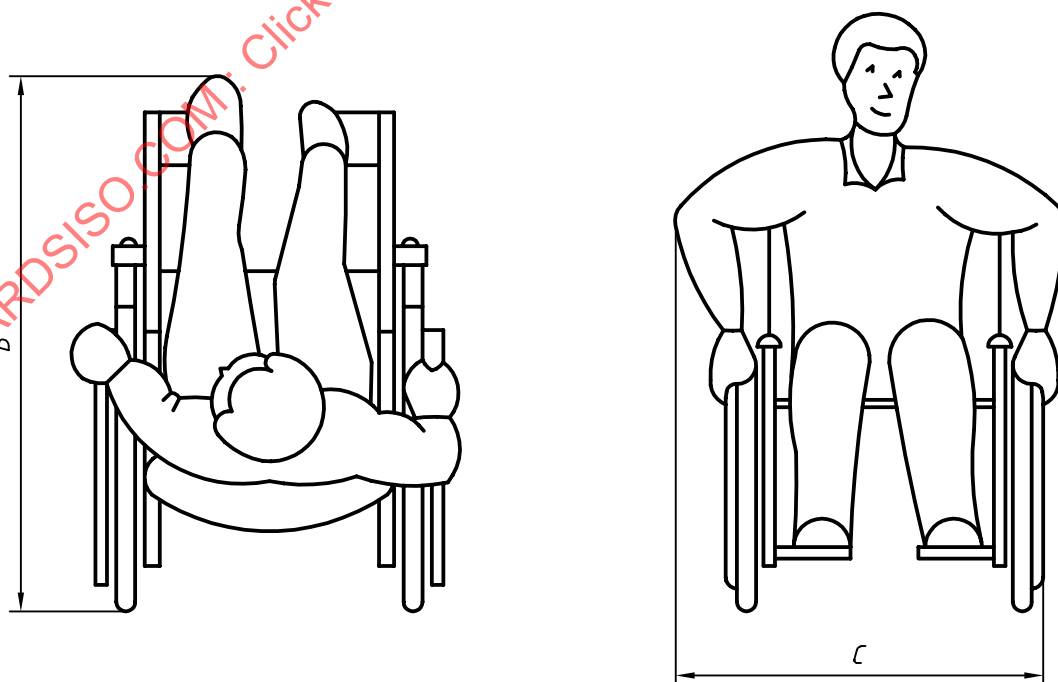
Figure 9 — Wheelchair clearance
