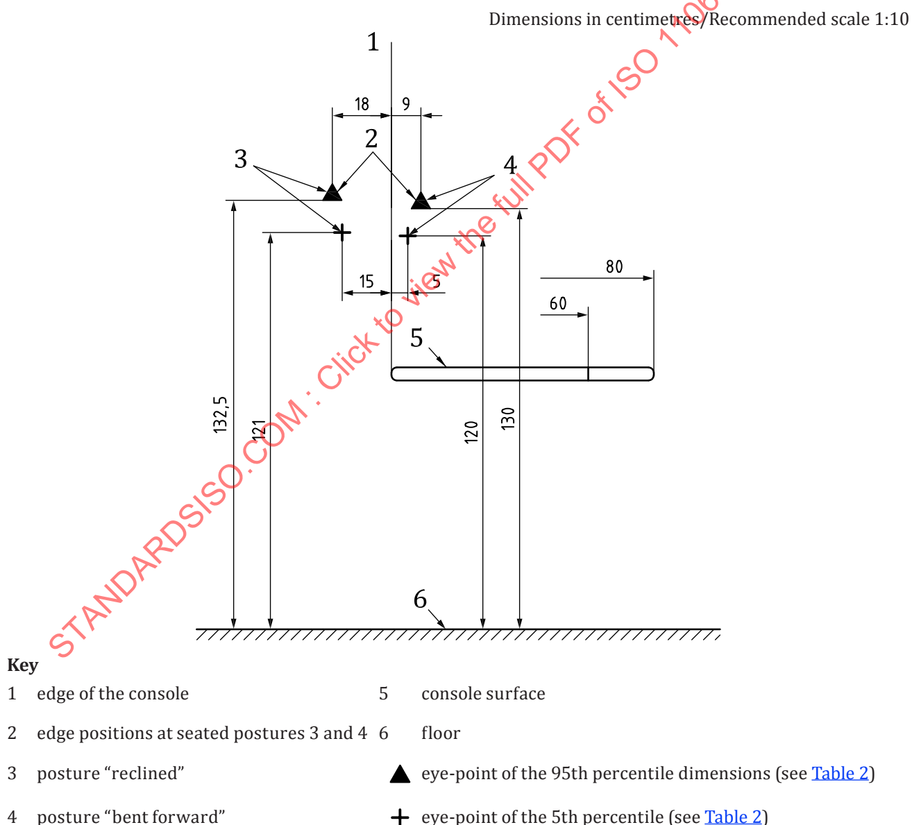
Figure A.3 — Template (example) — Console with eye-points — Elevation view
