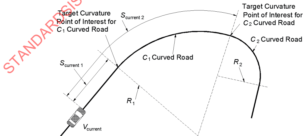
Figure 6 — Selection of the target curvature point of interest for multiple curve
