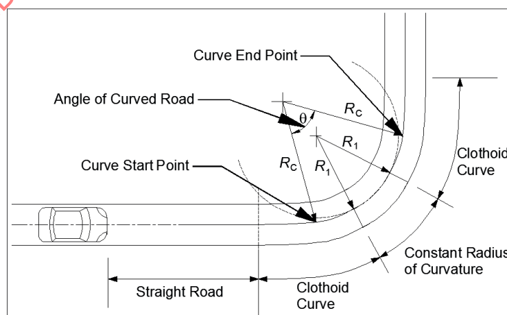
Figure 3 — Basic shape of a single curve with constant radius
