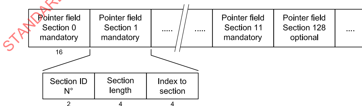
Figure 3 — Pointer section data part overview
