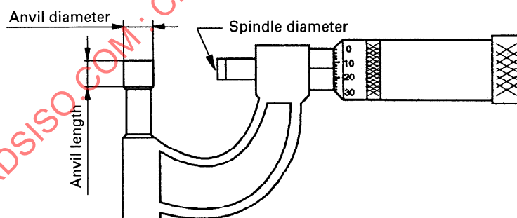
Figure C.2 — Example of wall-thickness micrometer
