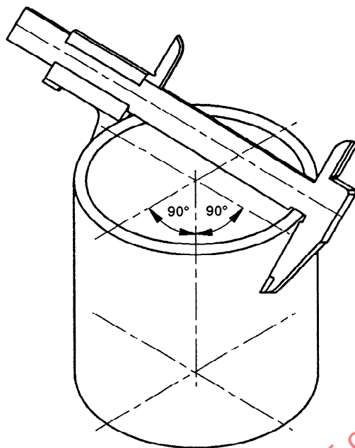
Figure 3 — Position of vernier calliper
