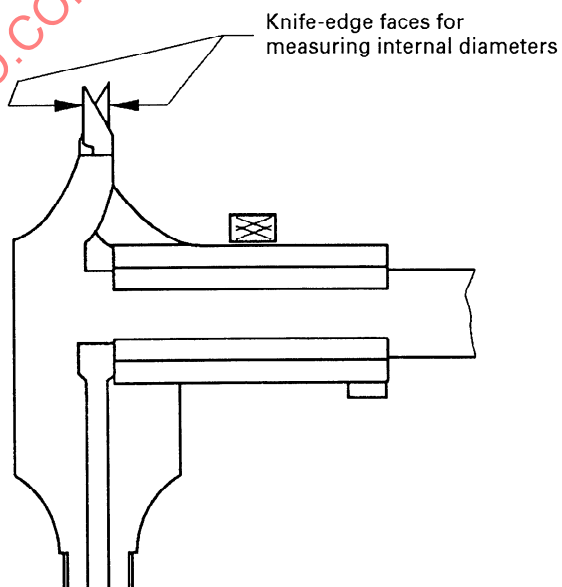
Figure B.2 — Type having jaws with knife-edge points
