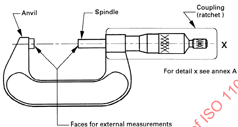
Figure C.1 — Example of external micrometer
