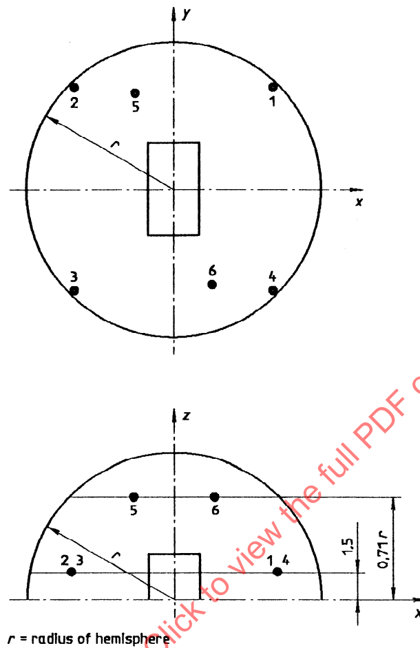
Figure 1 — Microphone positions on the hemisphere (see table 2)
