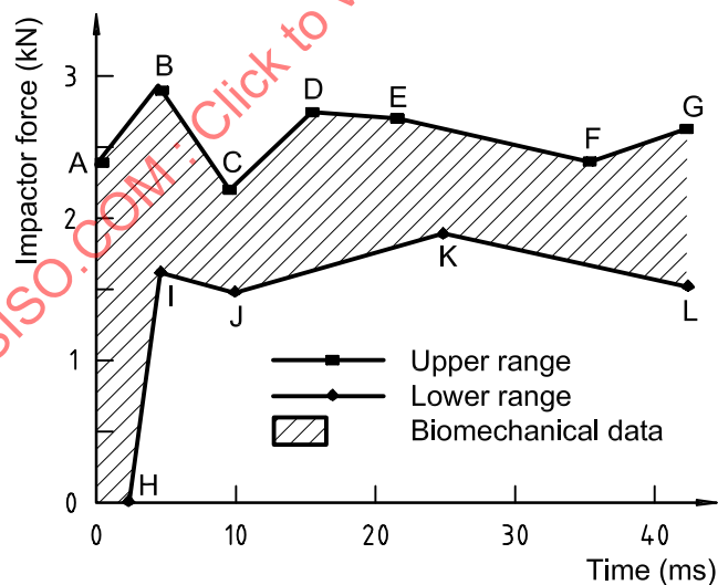
Figure A.5 — Force of bending test at 20 km/h
