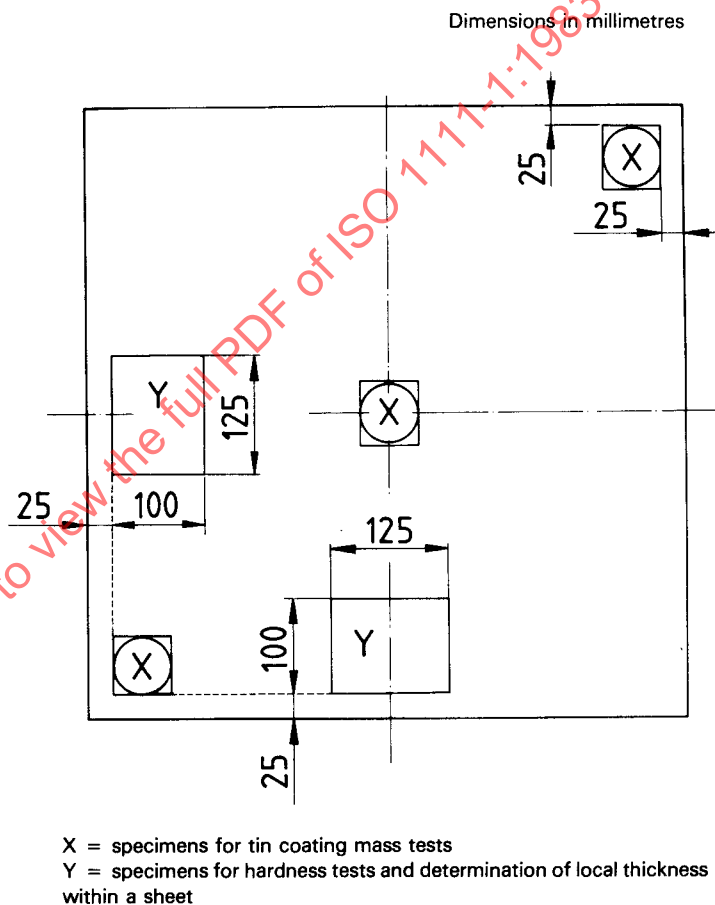
Figure 3 — Position of test specimens
