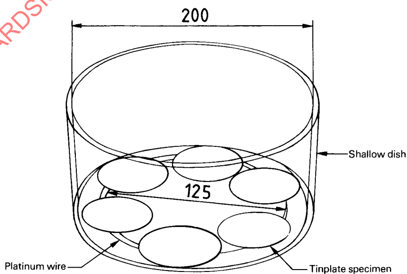
Figure 6 — Arrangement of specimens for dissolution of tin
