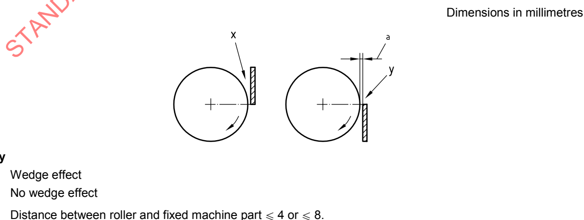
Figure 7 — Avoidance of wedge effect
