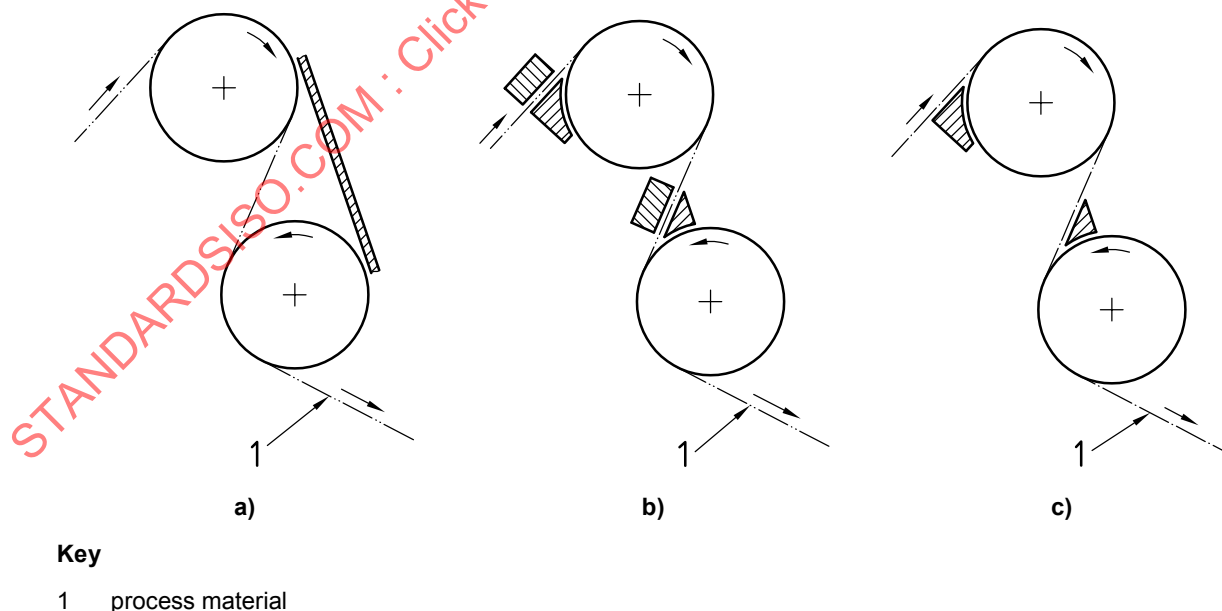
Figure 8 — Guards for on-running process material
