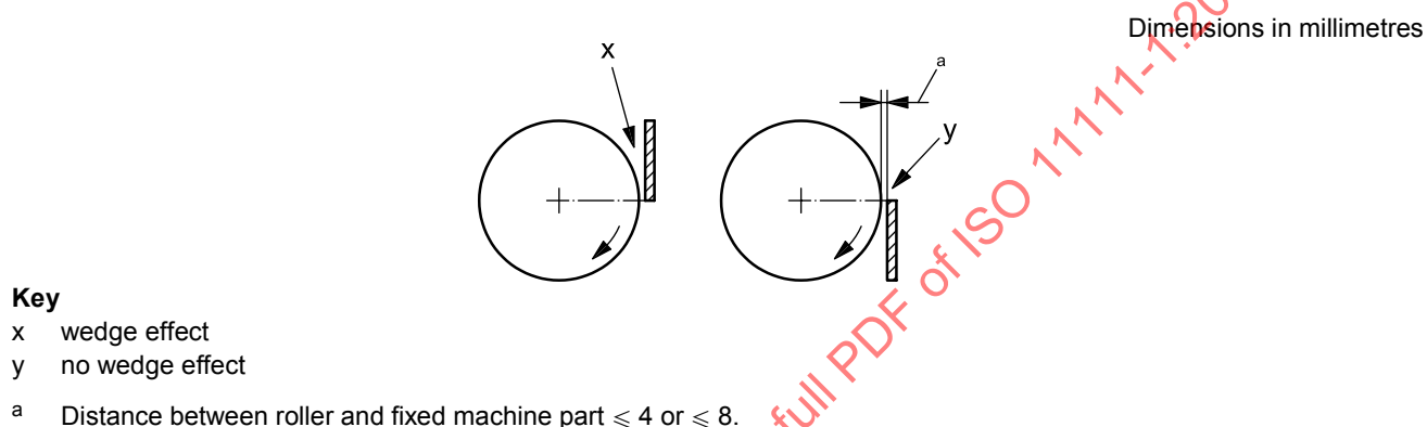
Figure 6 — Avoidance of wedge effect
