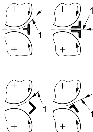
Figure 2 — Profiles of nip guards
