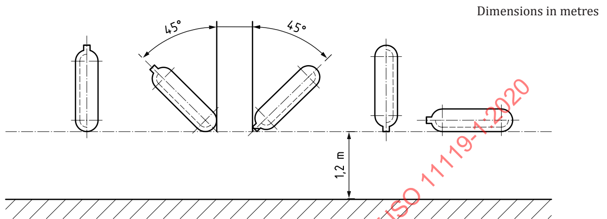
Figure 1 — Drop test
