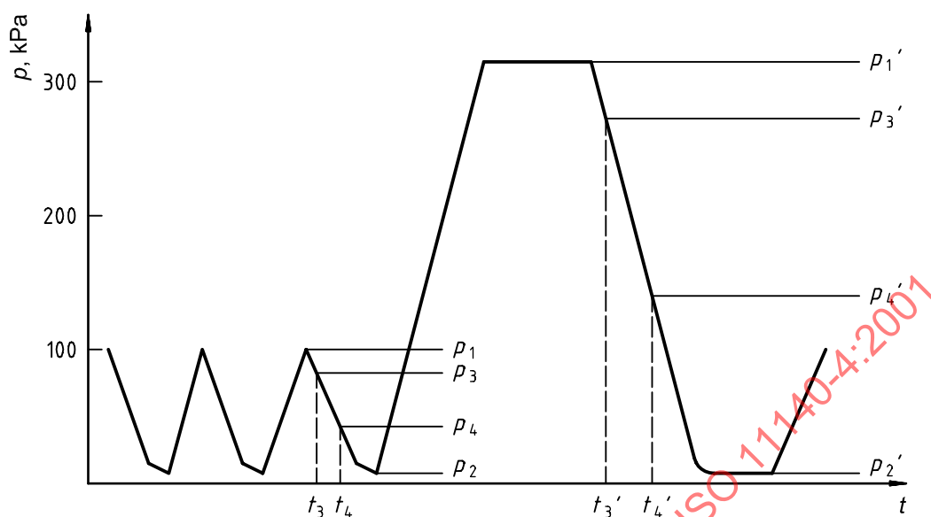
Figure A.1 — Determination of the rate of pressure change
