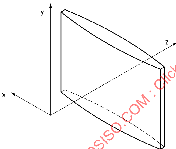
Figure 3 — Cylindrical lens in horizontally focusing orientation
