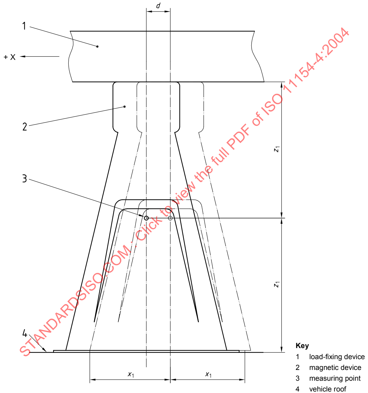
Figure C.1 — Measuring deflection, d
