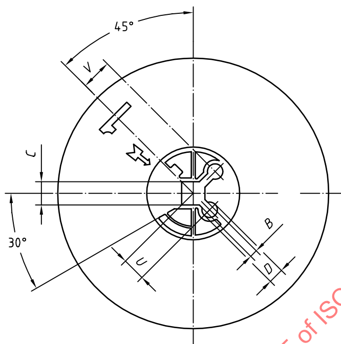
Figure 2 — Plastic spool
