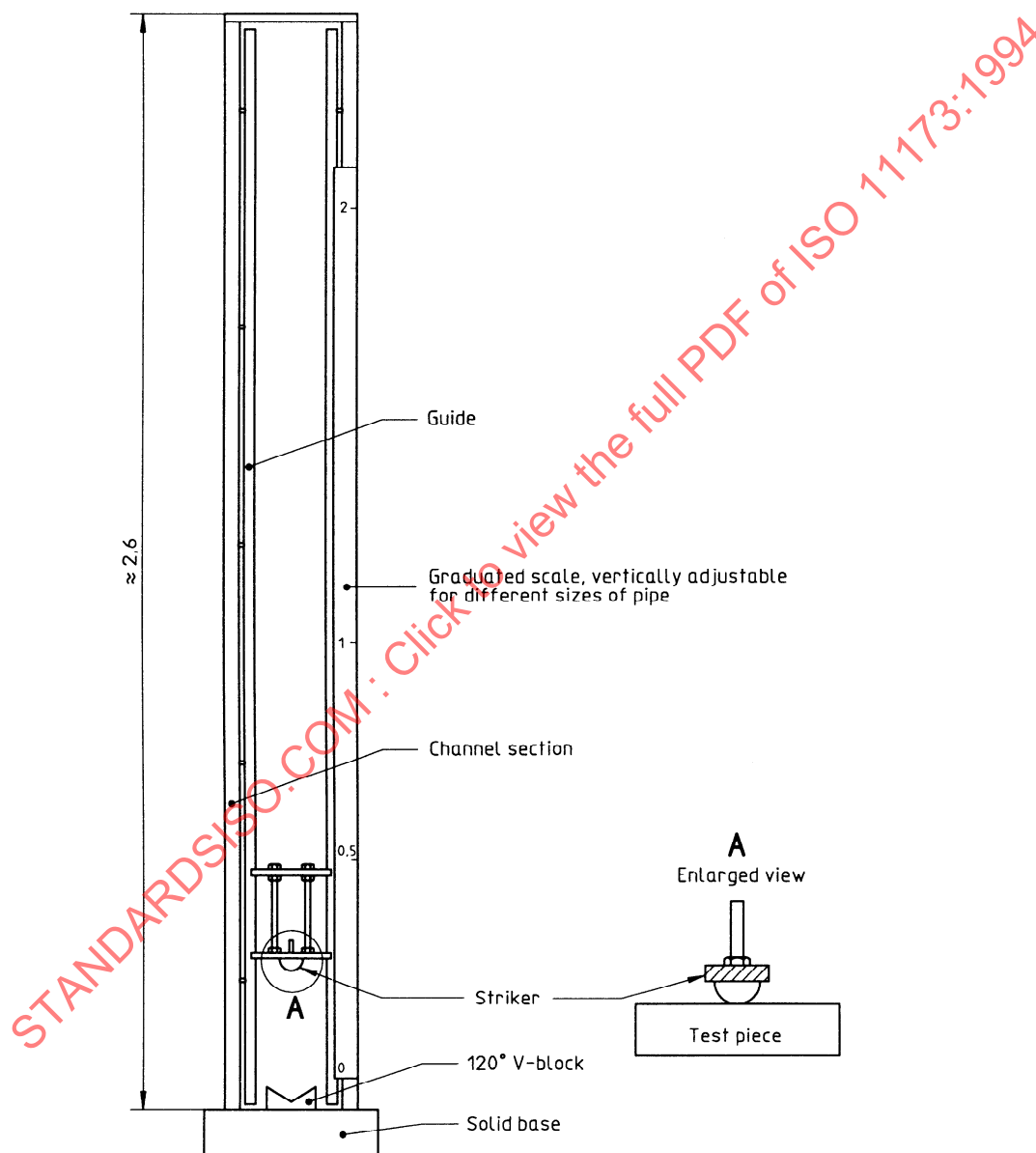
Figure 1 — Diagrammatic representation of an impact-testing machine
