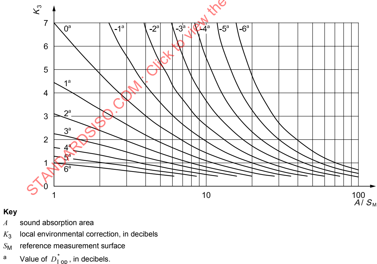
Figure A.2 — K_3 , in decibels, determined from A/S_M and D_{I \text{ op}}^* , being a graphical representation of Equations (A.5) and (A.6)
