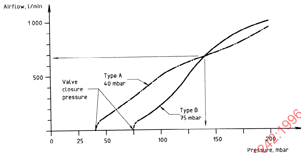
Figure B.2 — Typical valve characteristics airflow as a function of differential pressure
