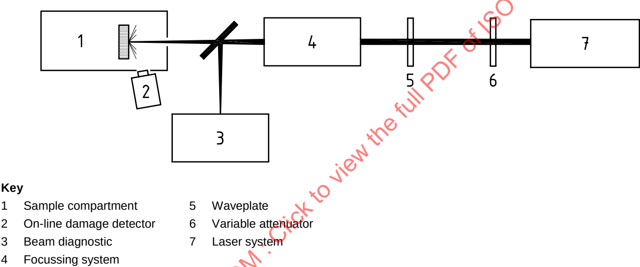
Figure 1 — Basic approach to 1-on-1 laser damage testing
