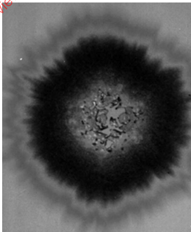
Nomarski micrograph for an energy density of 30 J/cm²
