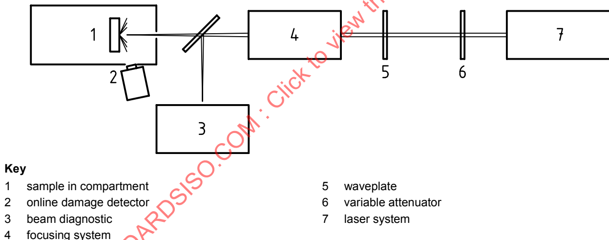
Figure 1 — Basic approach to laser damage testing
