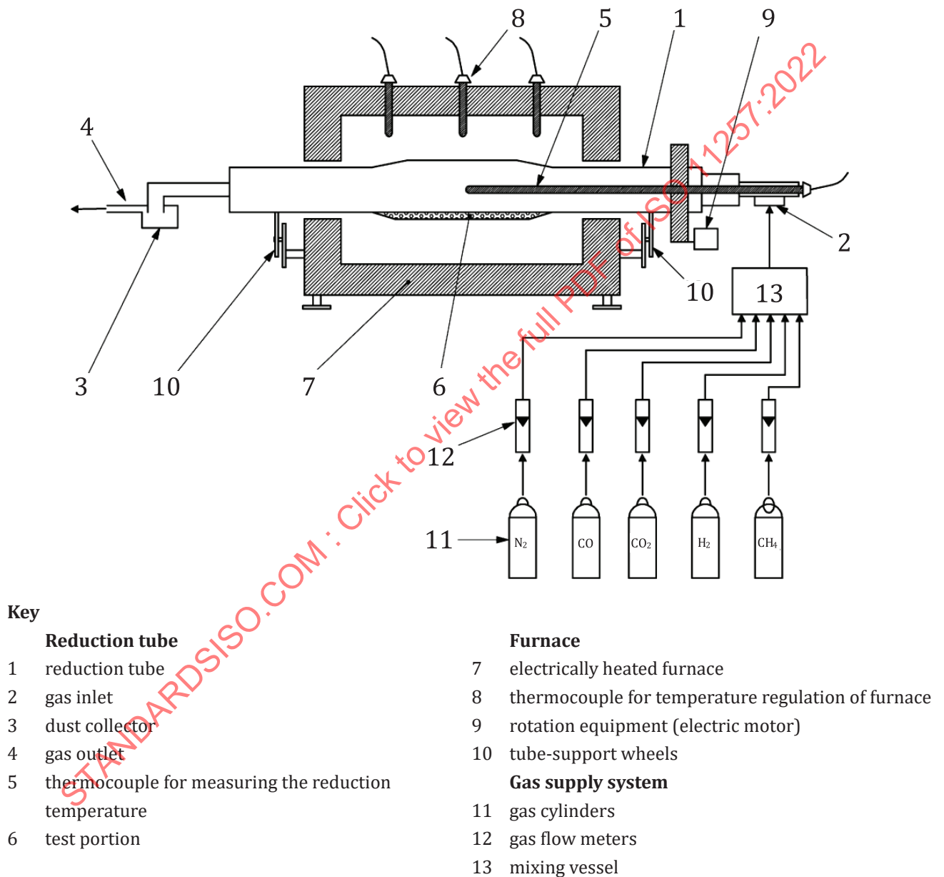
Figure 1 — Example of test apparatus (schematic diagram)
