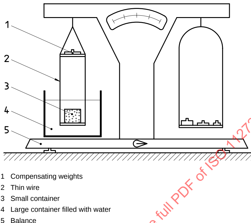
Figure 2 — Laboratory balance to determine the volume of clods by weighing in air and water
