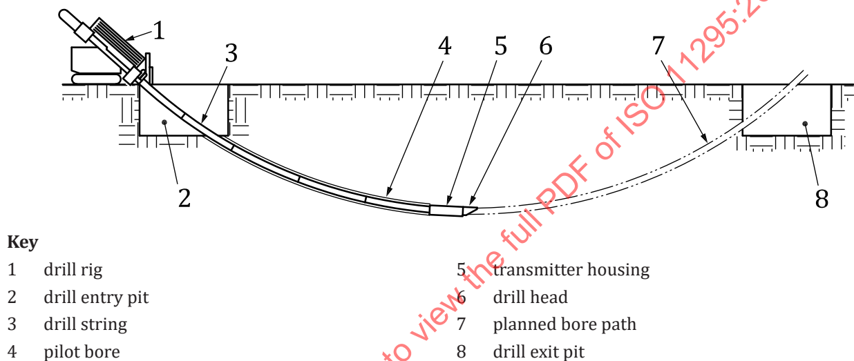
Figure 23 — Schematic representation of replacement by horizontal directional drilling — Pilot bore
