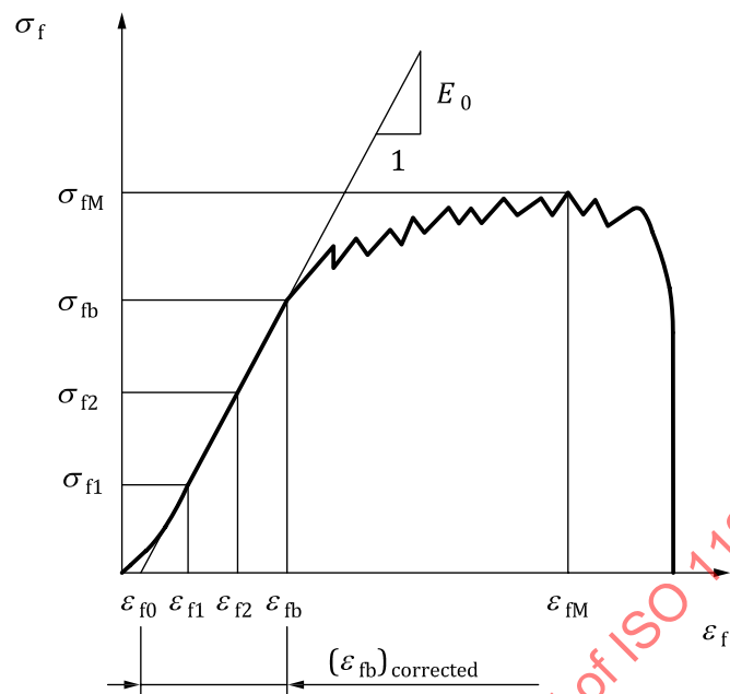
a) Composite with extensive strain capacity between first break and maximum applied load
