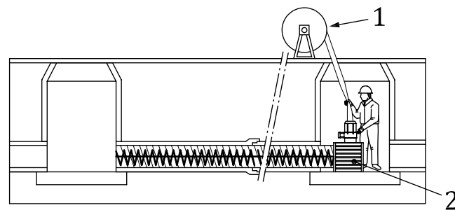
a) Method 1a: Fixed diameter from the manhole
