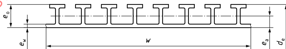
a) Example cross-section of a profiled plastics strip excluding locking mechanism forming the seam
