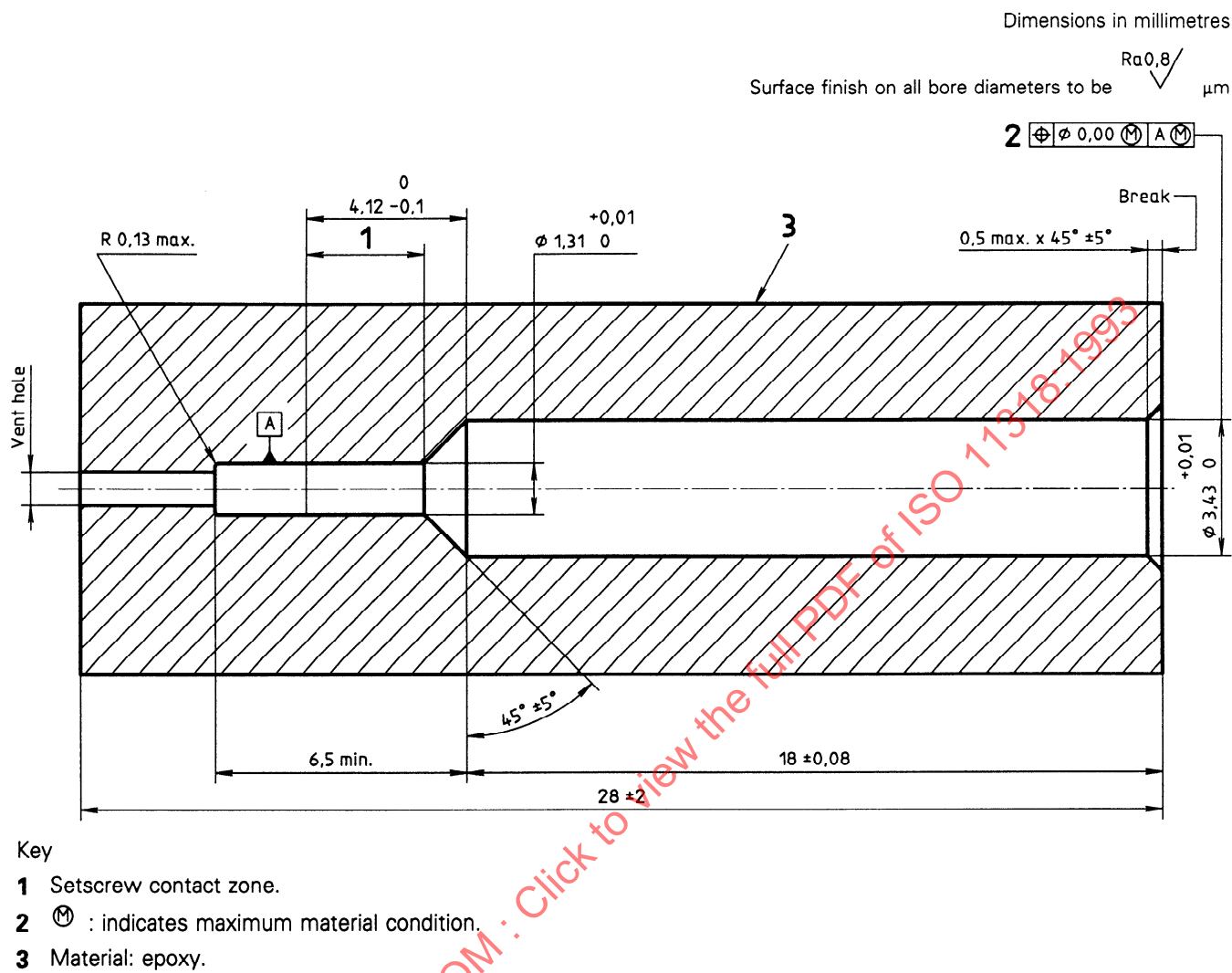
Figure 2 — DF-1 lead connector GO gauge
