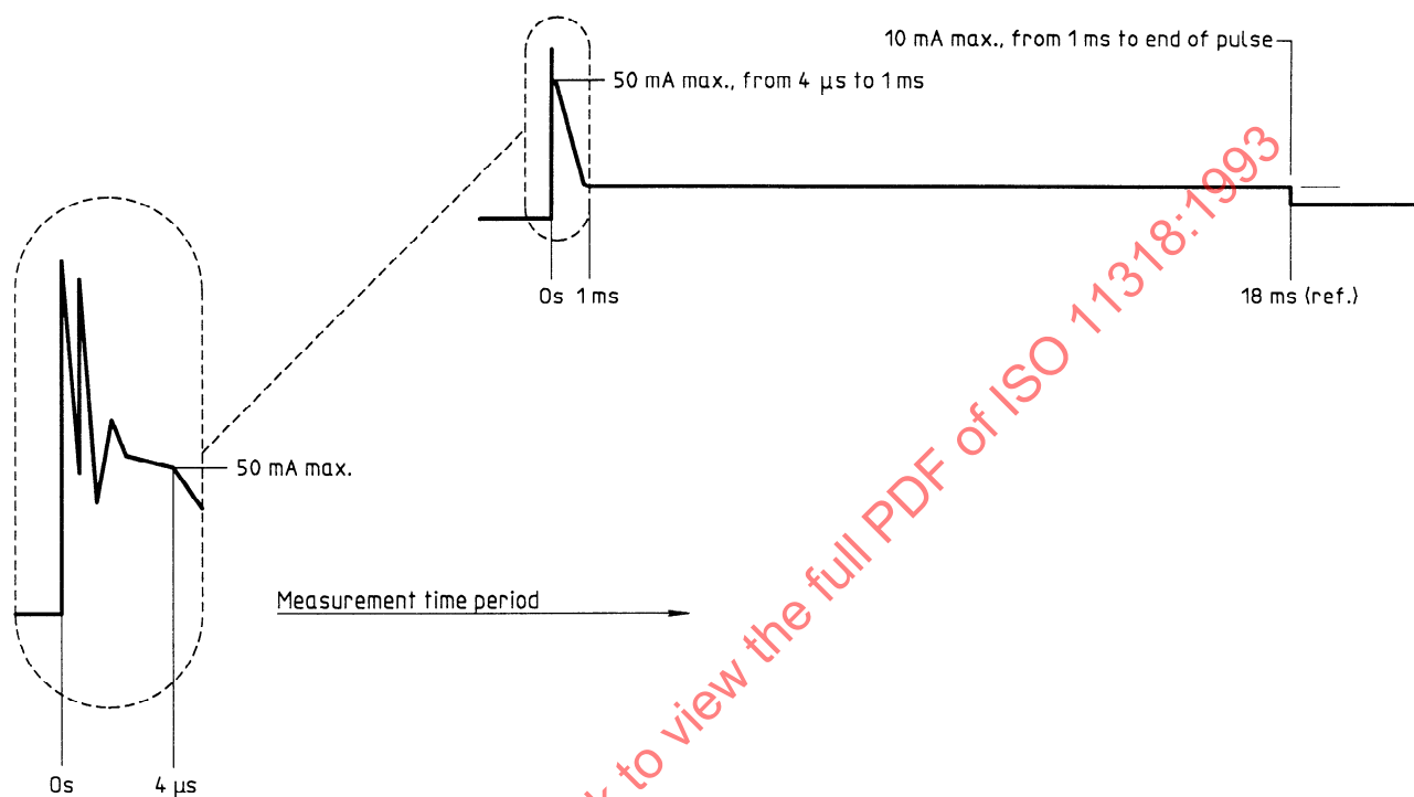
Figure A.5 — Current leakage waveform
