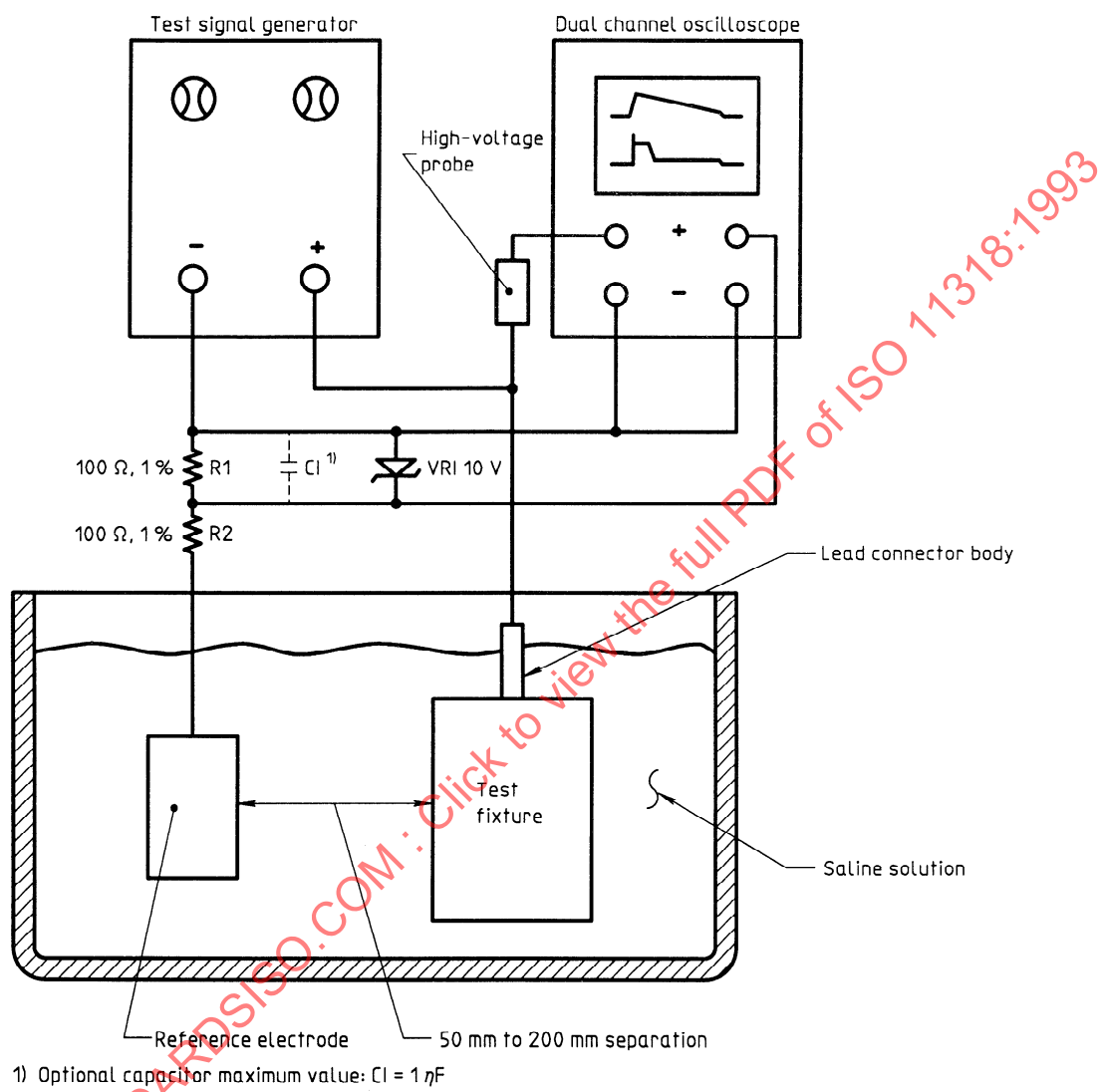
Figure A.1 — Electrical isolation test arrangement
