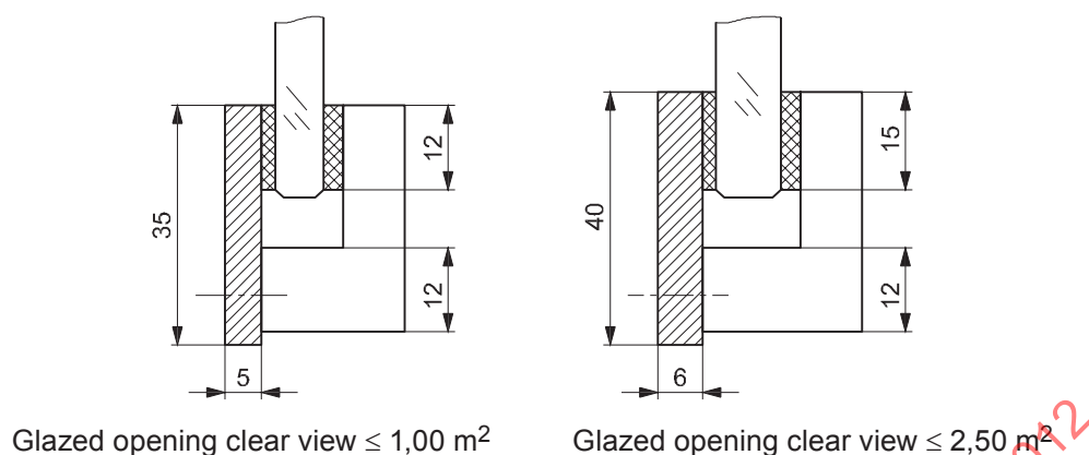
Figure 7 — Minimum dimensions (mm)
