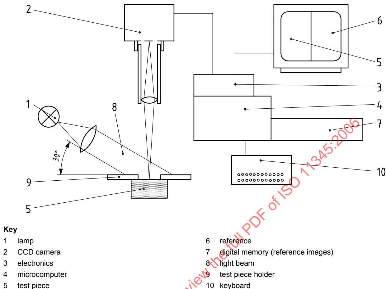
Figure 2 — Apparatus for methods B and D with a CCD camera
