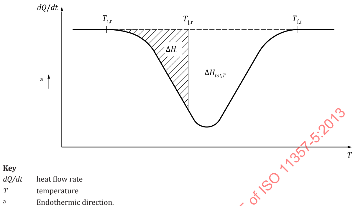
Figure 4 — Calculation of degree of conversion from a temperature scan
