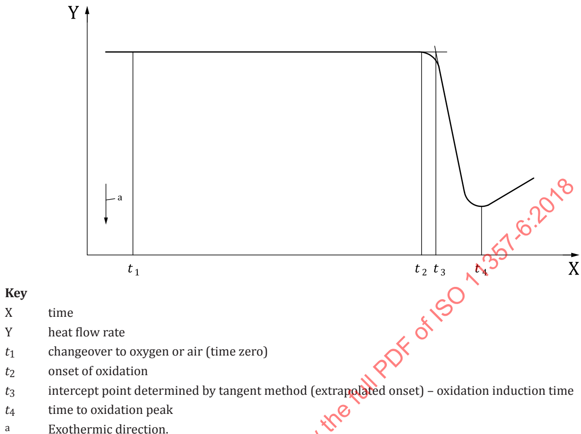
Figure 1 — Schematic oxidation induction time curve — Tangent method of analysis
