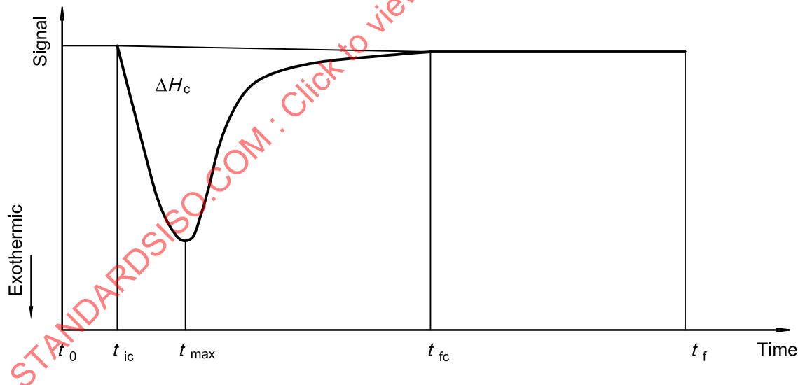
Figure 3 — DSC signal during the isothermal step
