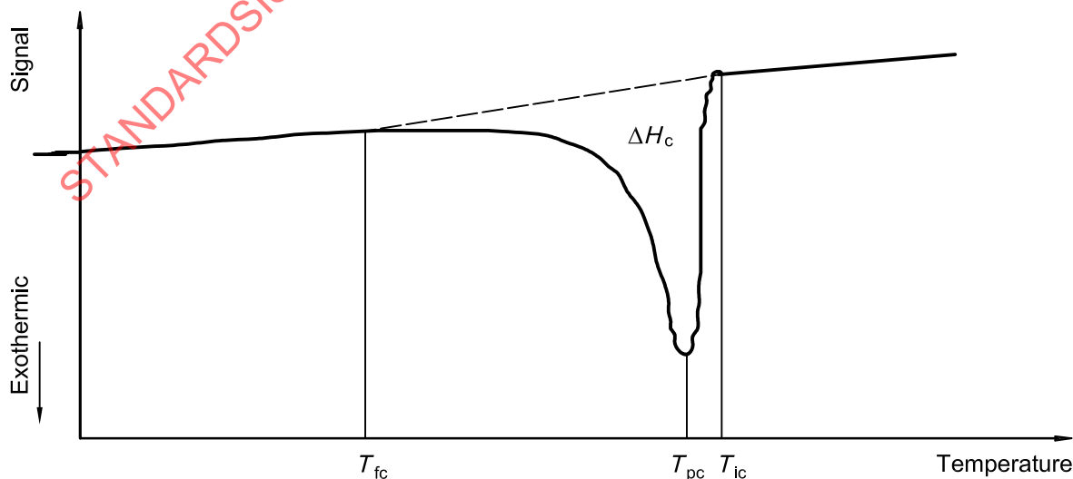
Figure 5 — DSC signal during the cooling step
