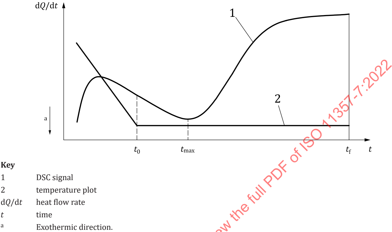
Figure 1 — Bad isothermal run — Crystallization started before isothermal temperature reached
