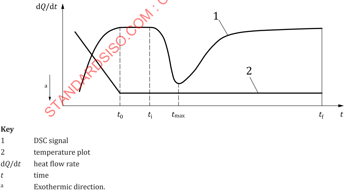
Figure 2 — Good isothermal run — Crystallization started after isothermal temperature is reached
