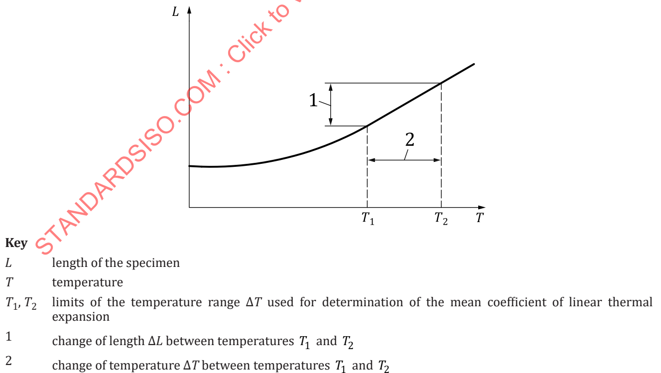
Figure 2 — Determination of mean coefficient of linear thermal expansion \bar{\alpha}
