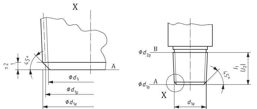
a) Valve stem thread profile
