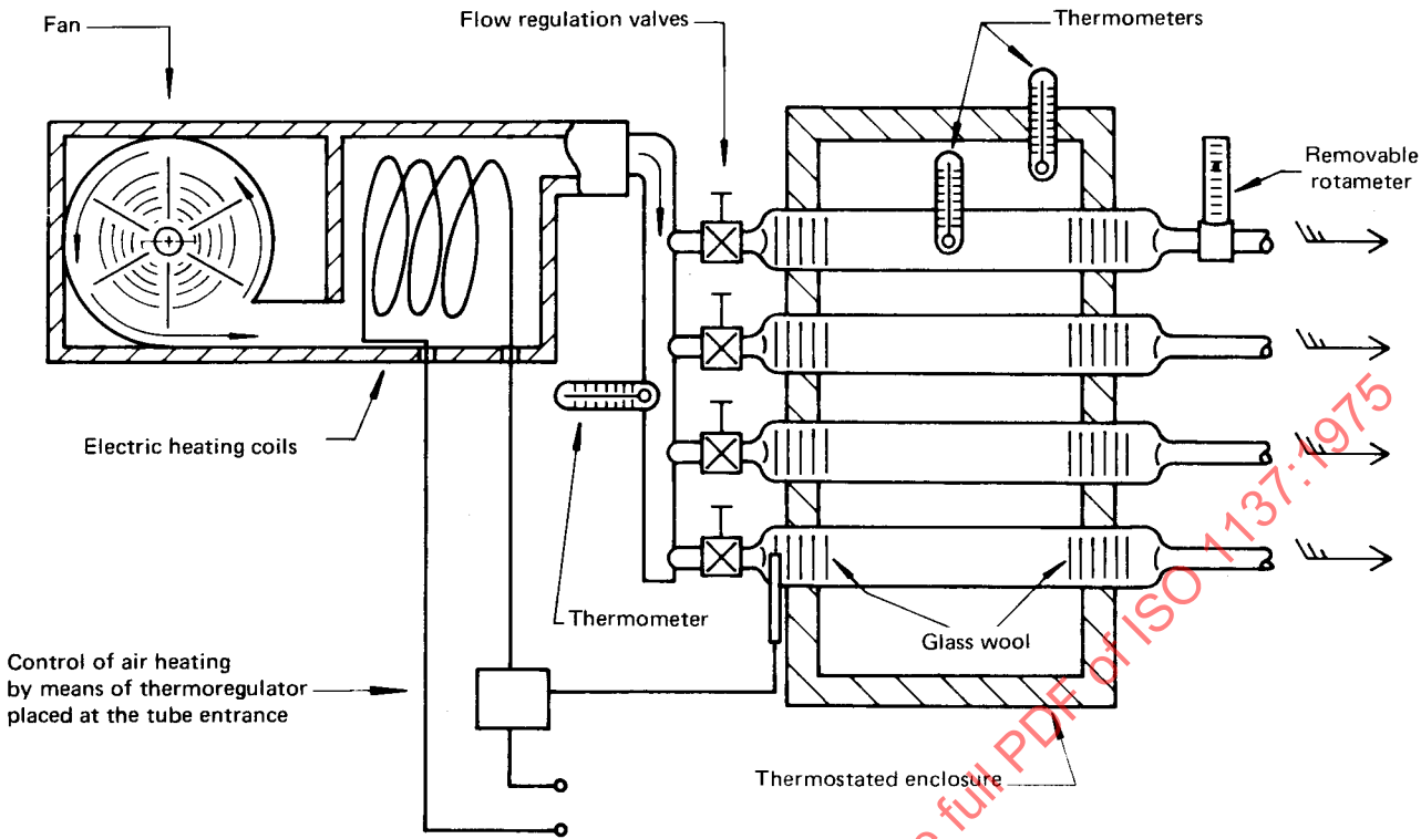
FIGURE 1 — General diagram of apparatus with horizontal tubes
