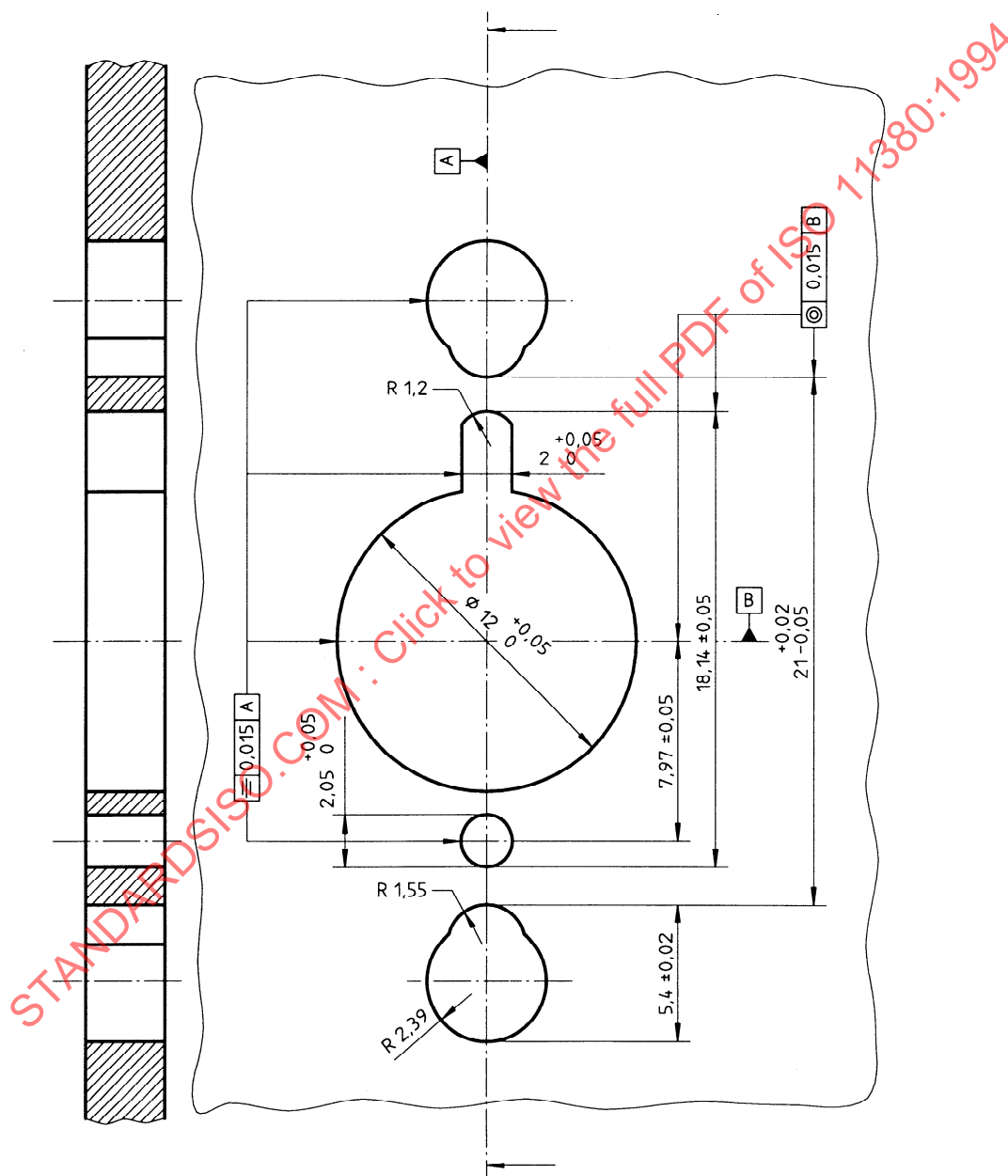
Figure 1 — Dimensions and tolerances
