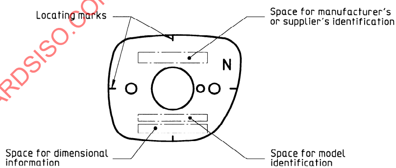
Figure 3 — Preferred locations of markings
