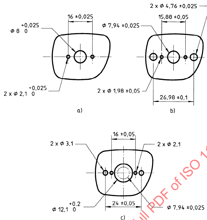
Figure 2 — Standardized system of holes
