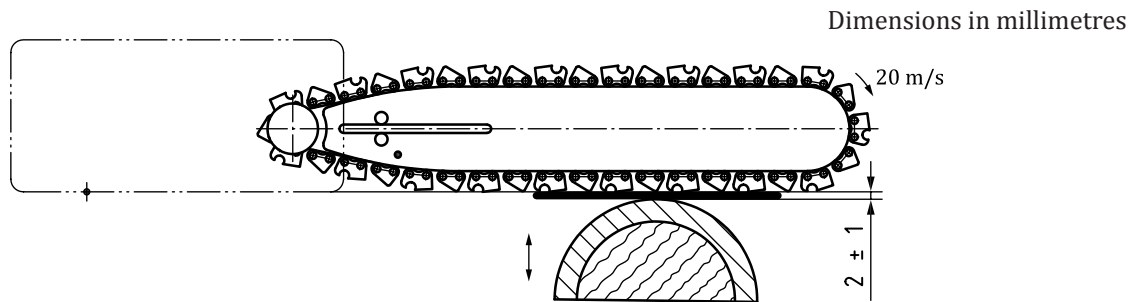
Figure 5 — Arrangement of test rig immediately before testing
