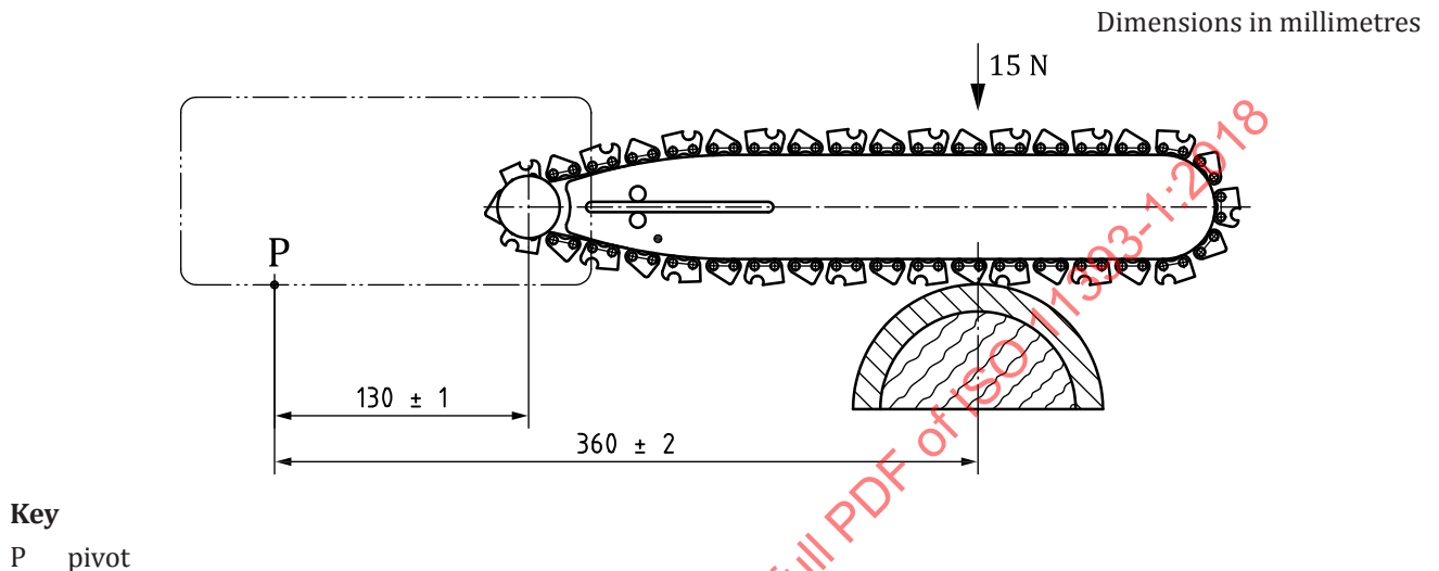
Figure 4 — Arrangement of test rig at time of cutting
