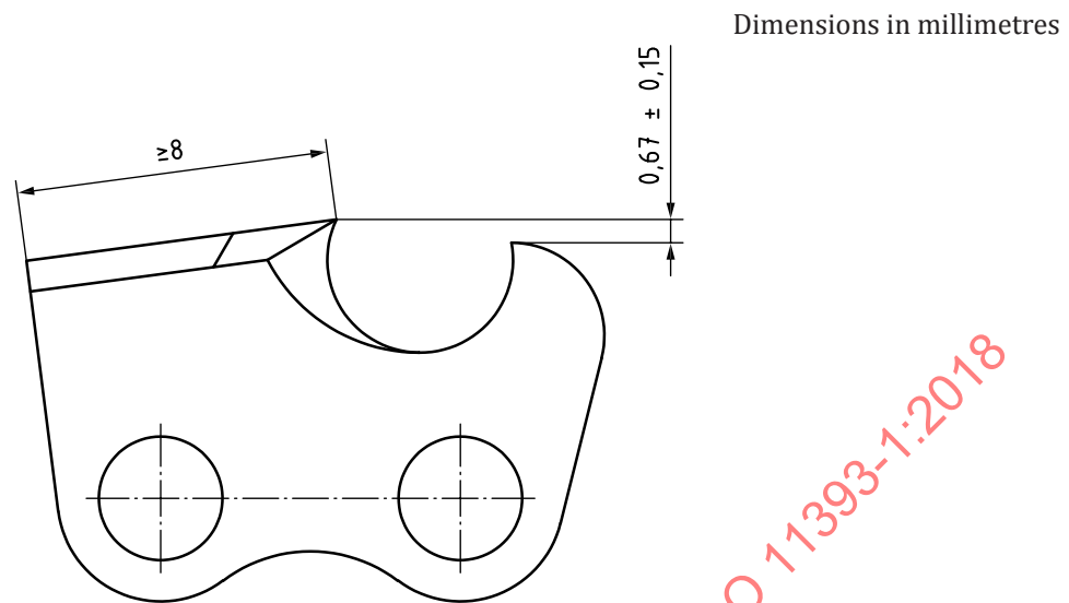
Figure 7 — Height of depth gauges of the cutter link
