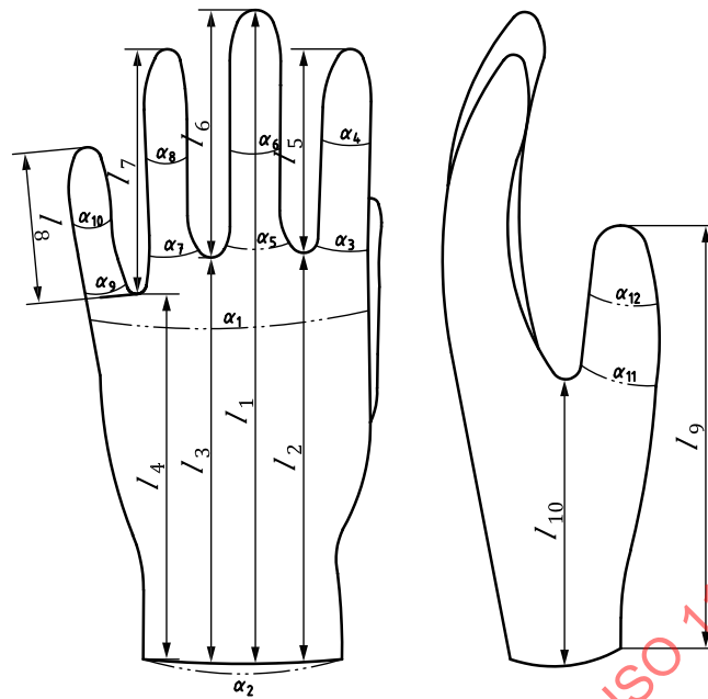
Figure 3 — Artificial left hand (the right hand is a mirror image)
